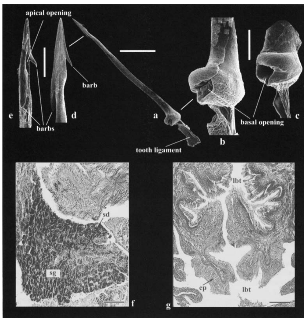
Fig. 3. Radula of Belaturricula gaini (Lamy, 1910) (a–e). a , single marginal tooth, scale bar = 200 mm, b , c , tooth base in two slightly different orientations to show the basal opening, scale bar = 50 mm, d , e , tooth tip in two different orientations to show the apical opening and barbs, scale bar = 50 mm, f , section through the salivary gland, g , section through the valvule. Scale bars = 200 mm. Abbreviations: ep = tall, columnar epithelium, lbt = lumen of the buccal tube, sd = salivary duct, sg = salivary gland.
